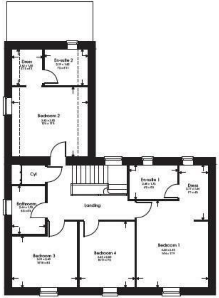
FIRST FLOOR
